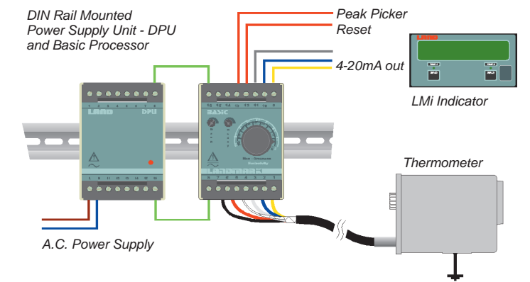
Landmark Basic Processor and DPU connections
